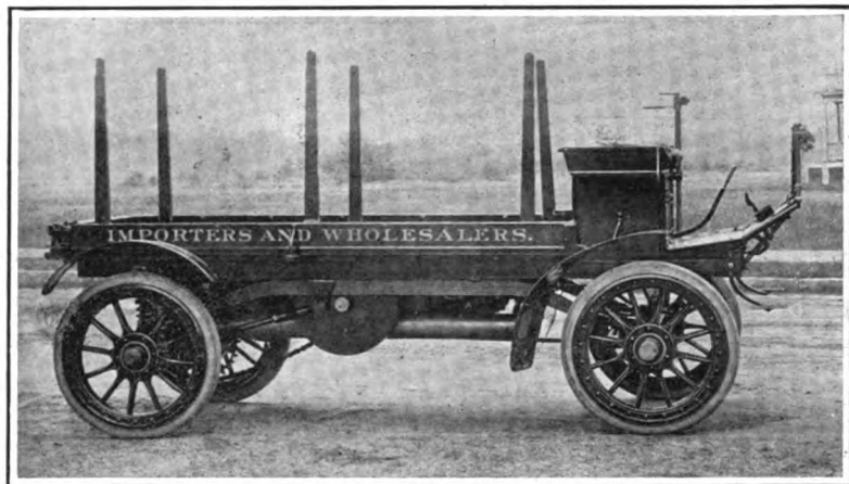
KNOX STAKE TRUCK BODY ON REGULAR DOUBLE-CYLINDER CHASSIS.
